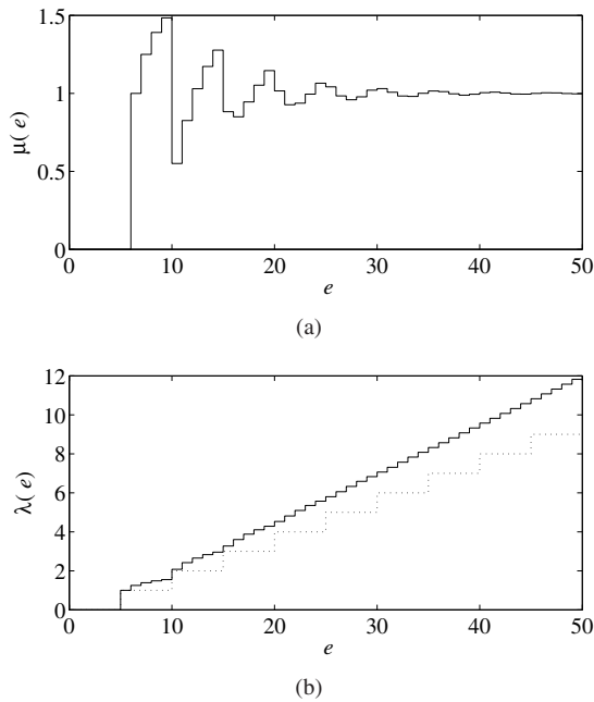
Fig. 2: The decision threshold (a) and the expected importance sum (b) (continuous line) as a function of the available energy. A uniform importance distribution U(0,2) with E_T = 4 and E_R = 1 is assumed. The stepwise function (dotted line) reflects the behavior of a non-selective transmitter, which transmits any message whatever its importance value is.
