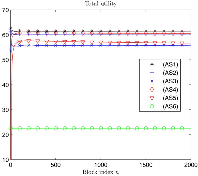
Fig. 1. Utility trajectories (as block index n varies) for different allocation schemes (AS).
